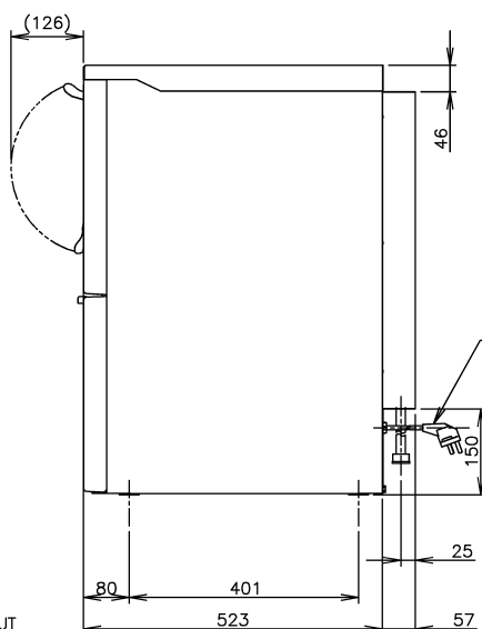
RIGHT SIDE
